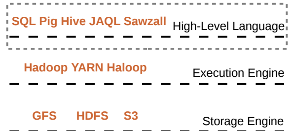
Fig. 2: Our logical workflow occupies the high-level layer of the generic MapReduce software stack for data processing.
