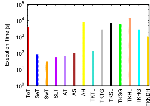
Fig. 6: The query execution times for the 100 GB data set. Logarithmic vertical axis.
