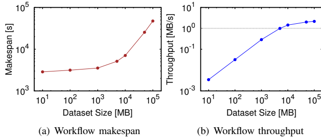
Fig. 4: The makespan and throughput for all input data sizes. The axes are logarithmic and do not start at 1.
