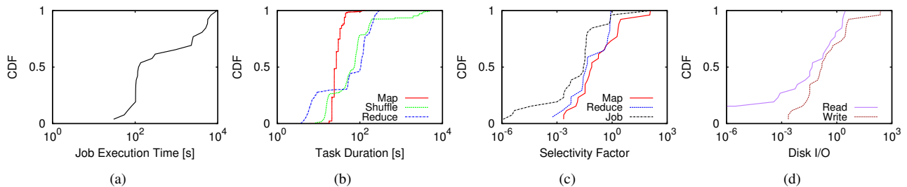
Fig. 7: The MapReduce job profiles: a) the job durations distribution, b) the task durations distribution, c) the task selectivity (ratio between output and input size), and d) the disk I/O (bytes read and written) between tasks, normalized by input size.
