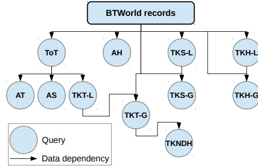
Fig. 3: The BTWorld logical workflow diagram. A data dependency is a form of inter-query dependency.
