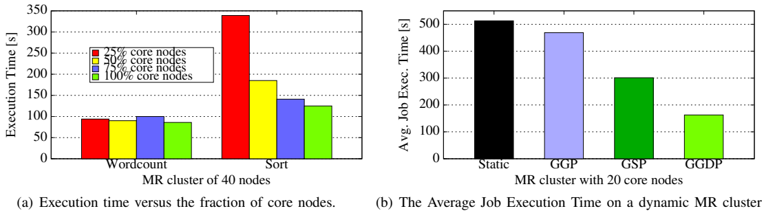
Figure 5. The MR-Runner performance under single and multiple jobs workloads.
