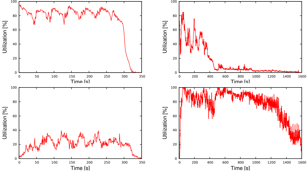
(c) Disk Utilization of Wordcount. (d) Disk Utilization of Sort. Figure 3. The CPU and disk utilization for the Wordcount and Sort applications.
