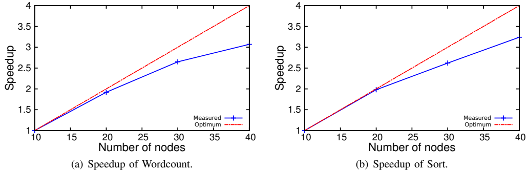
Figure 4. The speedup for the Wordcount and Sort applications on MR clusters with only core nodes.
