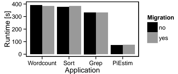
Fig. 3. The job runtime without migration versus the job runtime with migration across two partitions in a 20-worker Hadoop framework.
