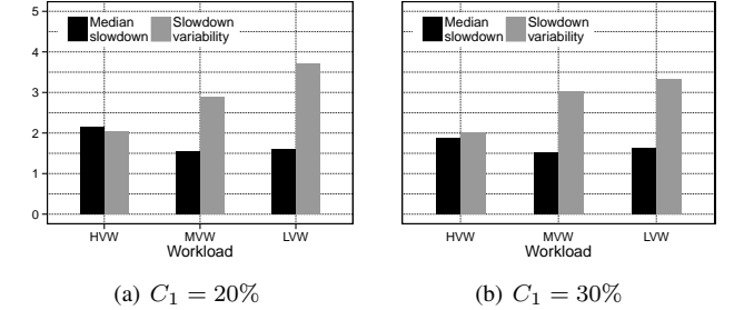
Fig. 9. The median job slowdown and the job slowdown variability versus the workload variability with STATICTAGS.
